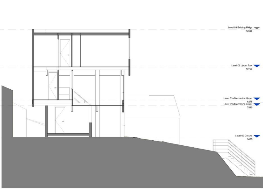
1 Existing Section 1:50
