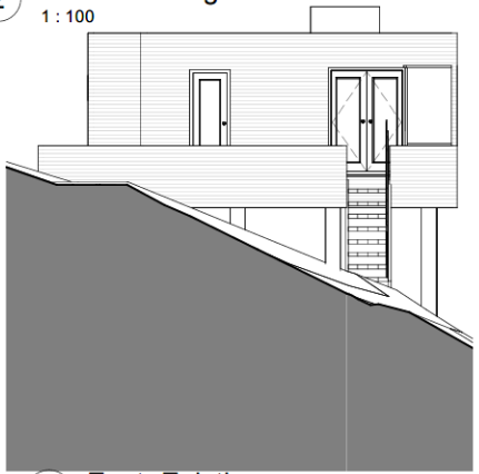
④ East- Existing 1 : 100
