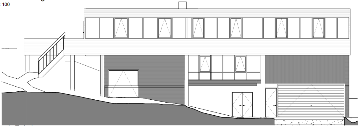
③ North Existing 1 : 100
