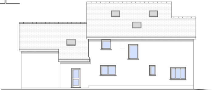
Rear Elevation
