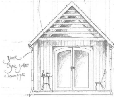
FRONT ELEVATION ~ SOUTH ~
