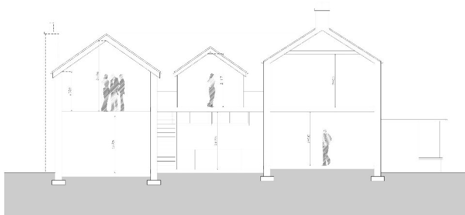
Section BB
