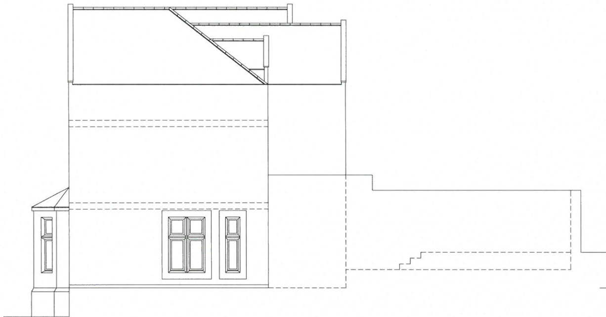
SIDE ELEVATION
