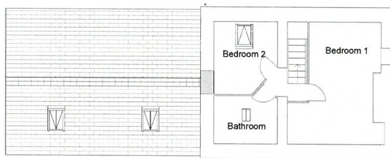
2 Level 1 - Proposed 1 : 100
