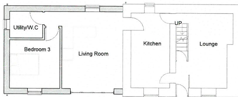
1 Level 0 - Proposed 1 : 100
